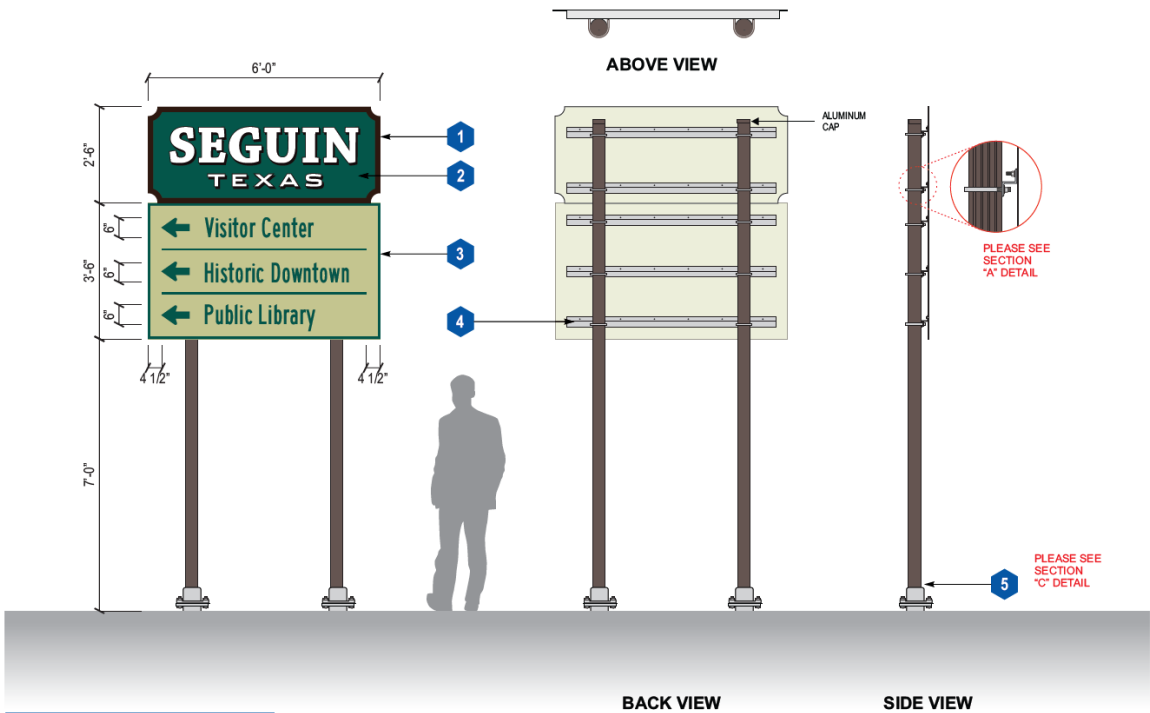
002 VEHICULAR SIGN SCALE: 3/8" = 1'
