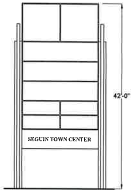
PYLON SIGN TYPE _A1
