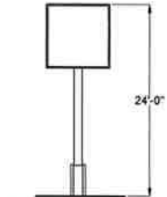
PAD POLE SIGN TYPE _D1
